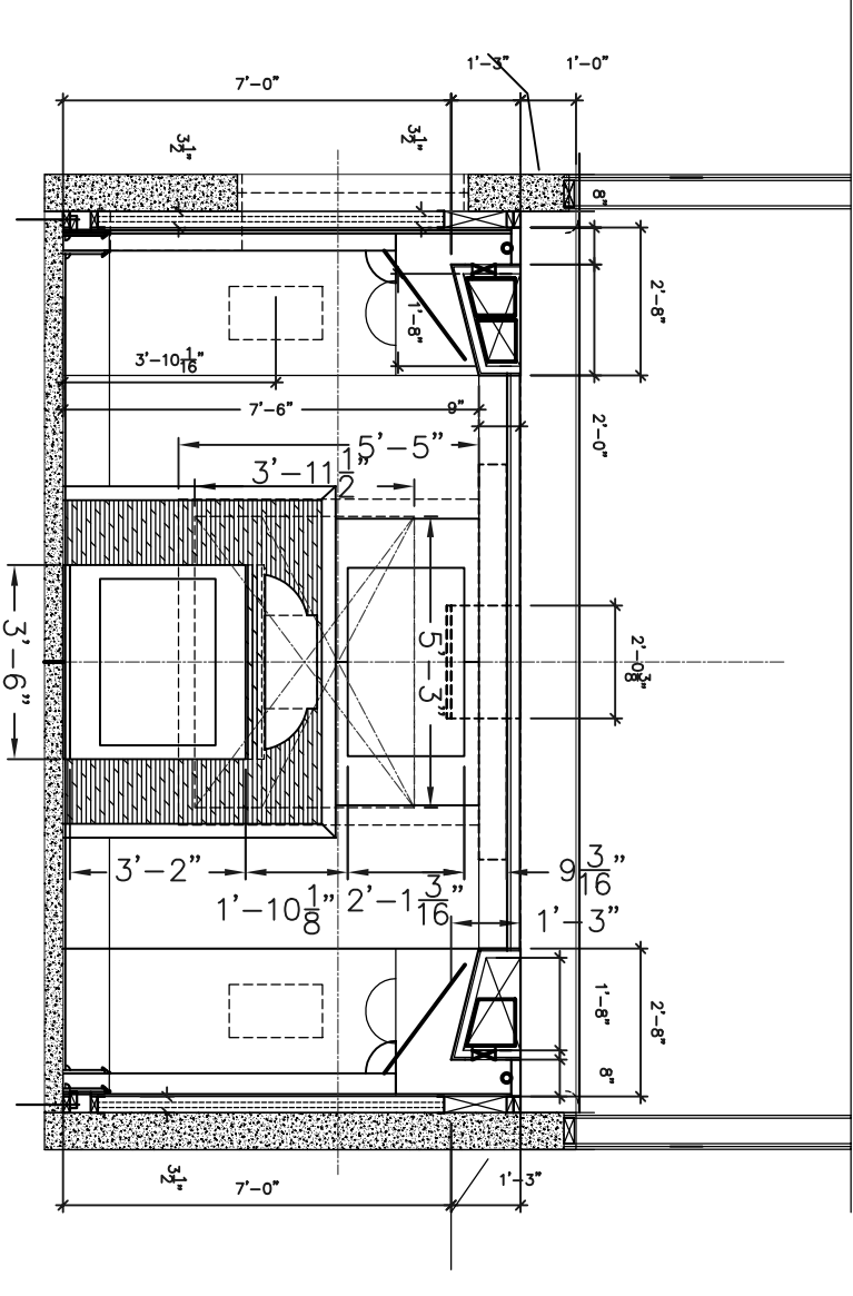
2 THEATER CROSS-SECTION - NORTH WALL
